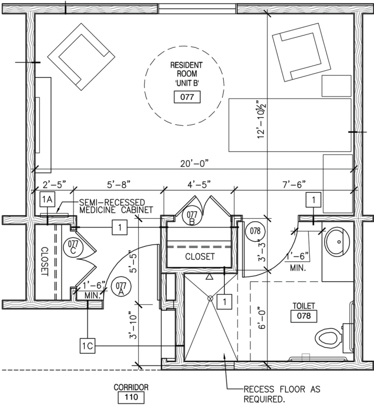
D3 ENLARGED PLAN - RESIDENT ROOM B SCALE: 1/4" = 1'-0" 440 Square Feet
