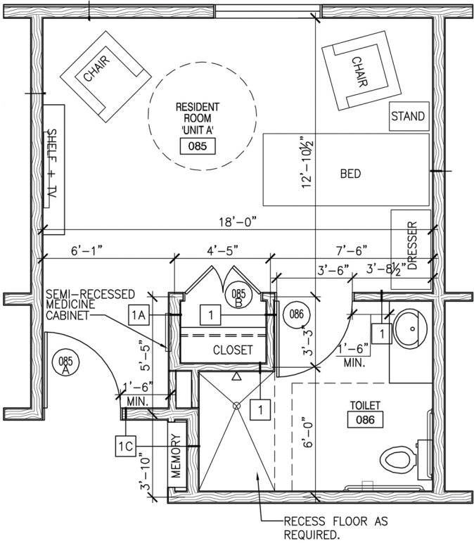
D1 ENLARGED PLAN - RESIDENT ROOM A SCALE: 1/4" = 1'-0" 360 Square Feet
